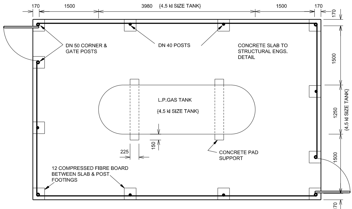
PLAN
