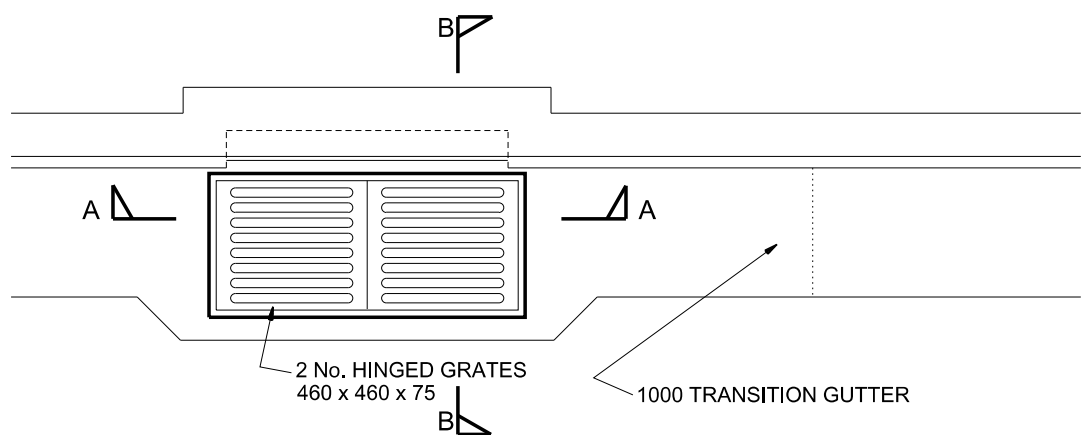
PLAN - DOUBLE GRATED GULLY PIT
