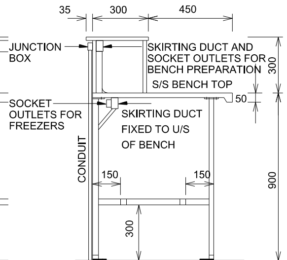
SECTION TYPICAL - BENCH PREPARATION
