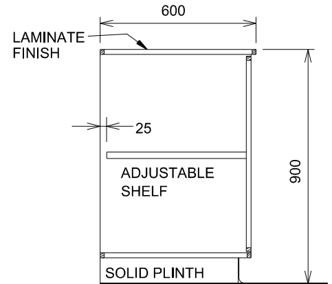
SECTION TYPICAL - BENCH CUPBOARD
