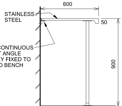
SECTION TYPICAL
