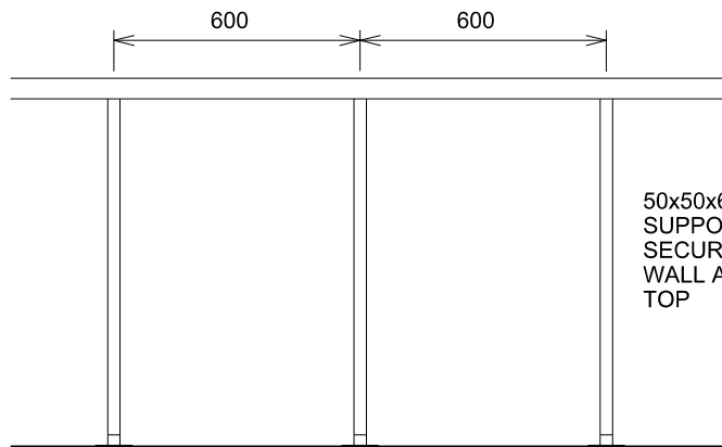
PART ELEVATION - BENCH PREPARATION AGAINST WALL
