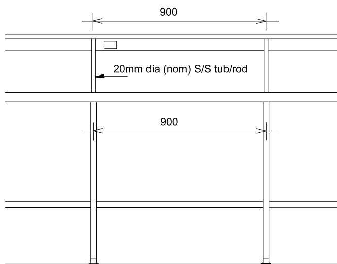
PART ELEVATION - BENCH PREPARATION
