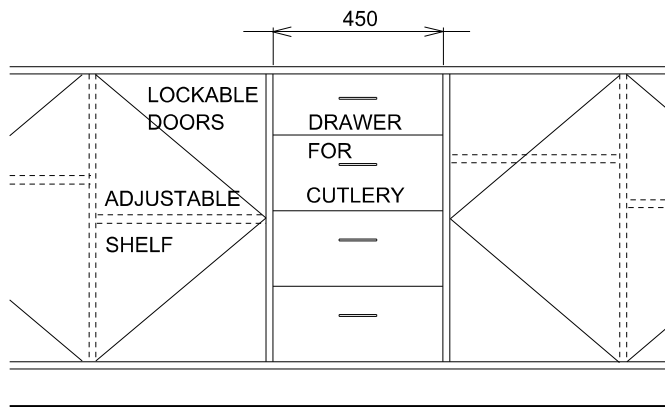
PART ELEVATION - BENCH CUPBOARD
