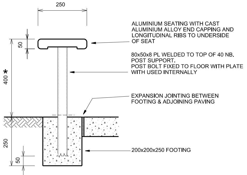
SECTION TYPICAL
