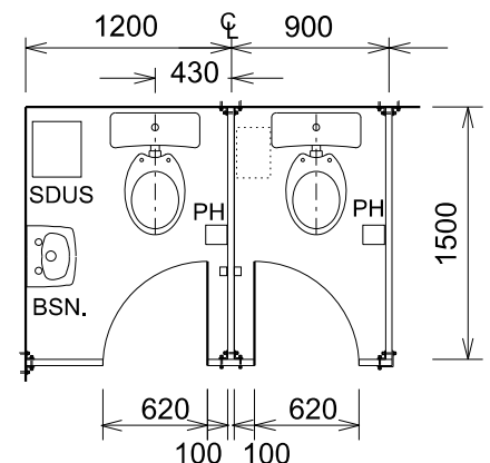
PLAN - W.C. WITH SANITARY DISPOSAL UNIT SERVICE NTS
