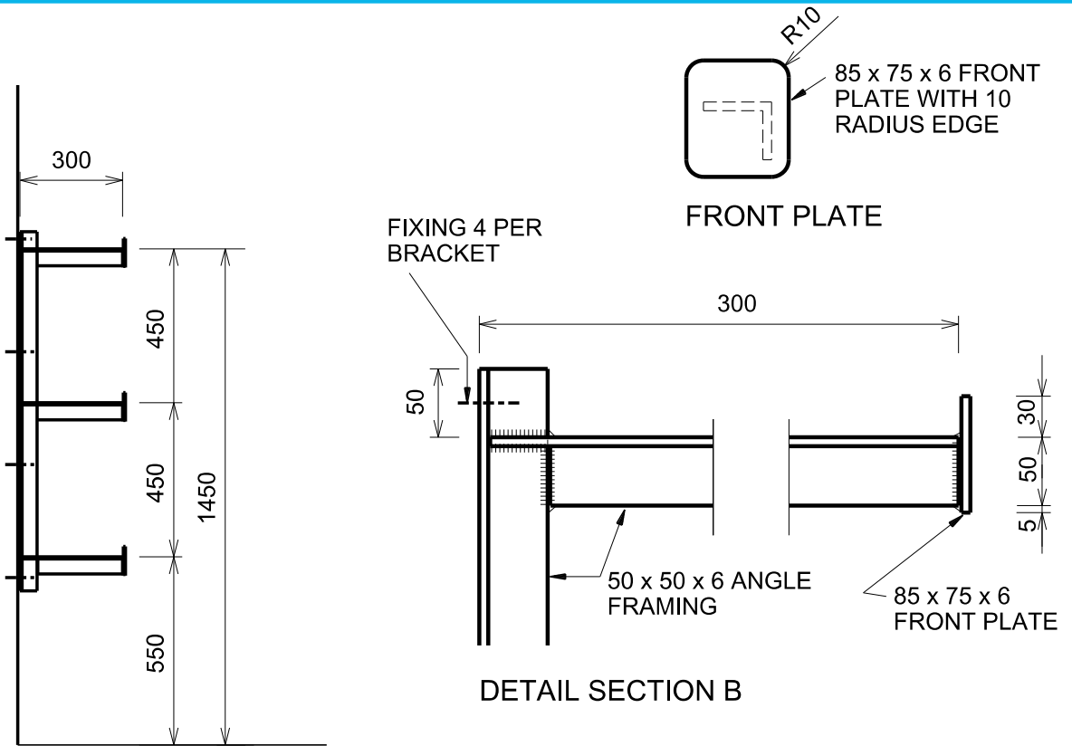
ELEVATION - IRRIGATION PIPE SUPPORT
