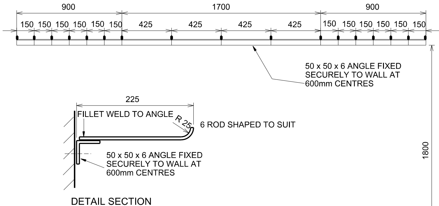
ELEVATION - IRRIGATION PIPE SUPPORT
