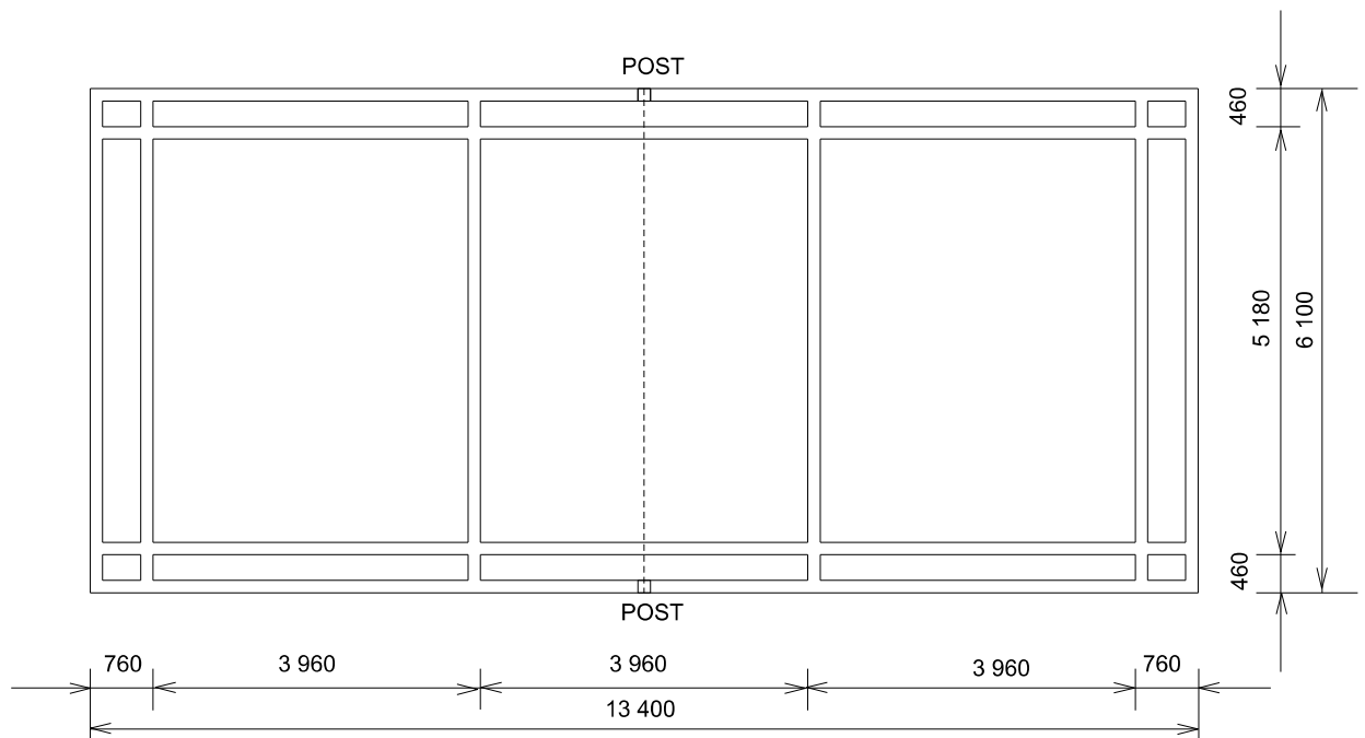
BADMINTON COURT DIMENSIONS
