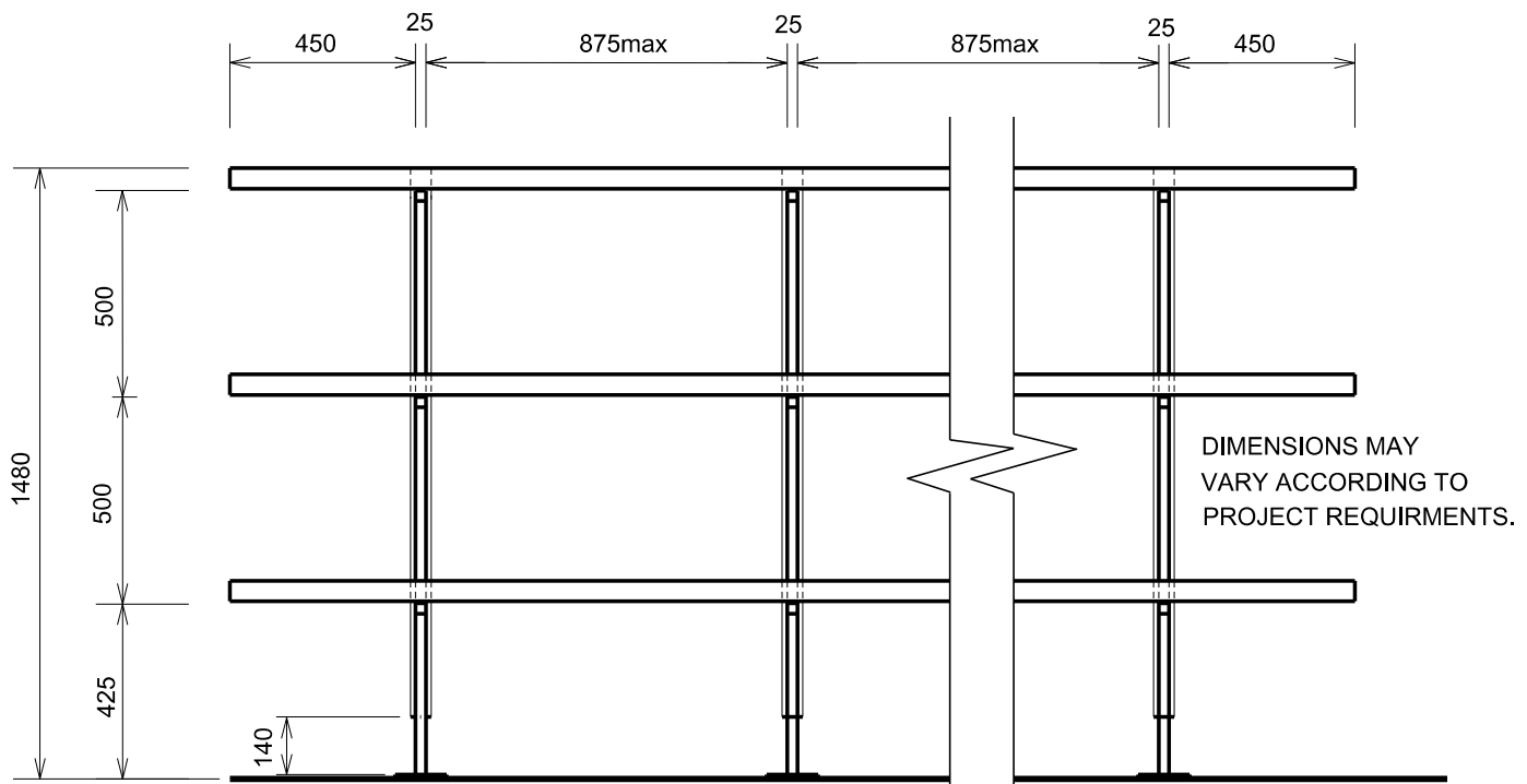
ELEVATION OF THREE TIER BAG RACK
