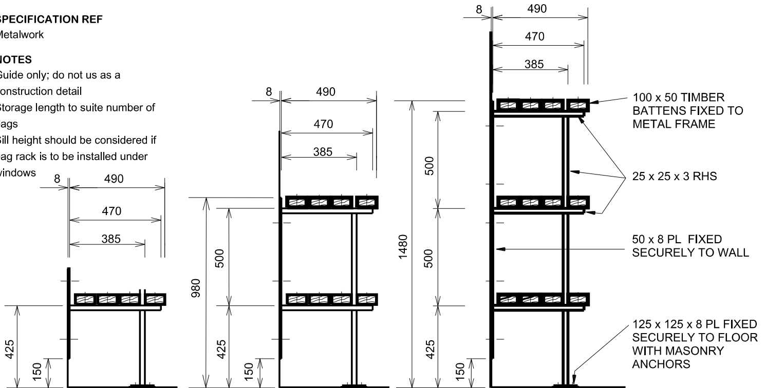
SECTION THROUGH ONE TIER BAG RACK
