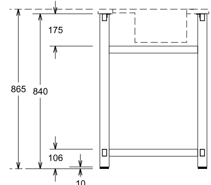
SUPPORT FRAME - SECTION THROUGH TROUGH
