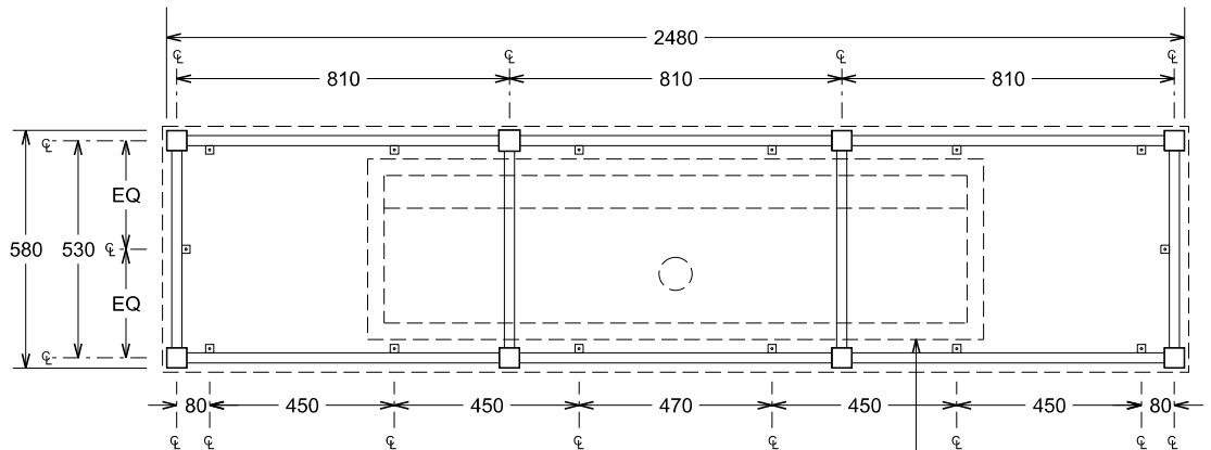
SUPPORT FRAME - PLAN
