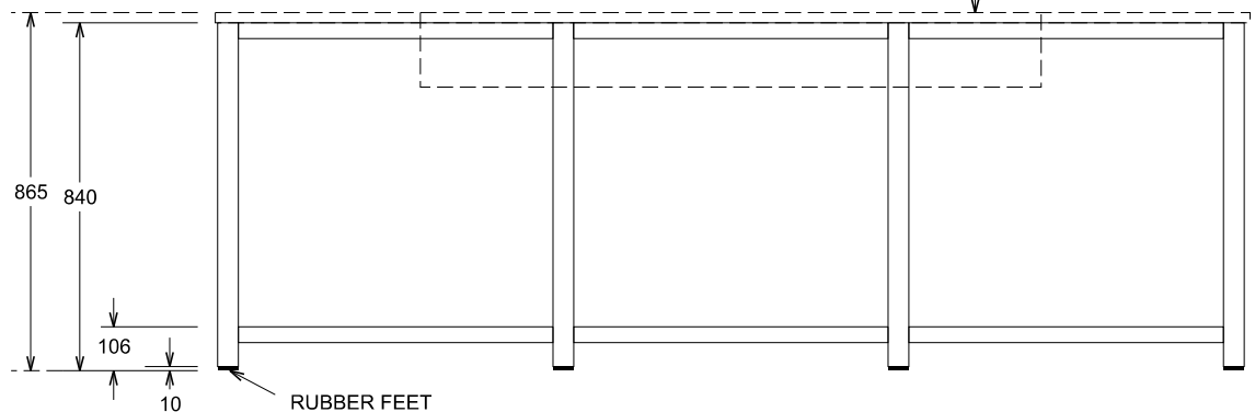
SUPPORT FRAME - FRONT ELEVATION
