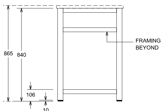
SUPPORT FRAME - END ELEVATION
