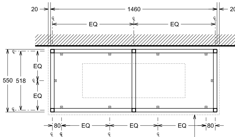
SUPPORT FRAME - PLAN
