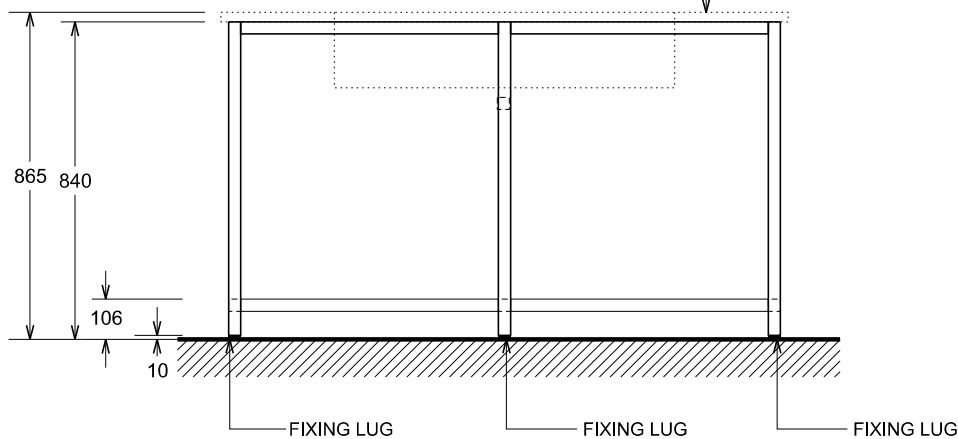
SUPPORT FRAME - FRONT ELEVATION
