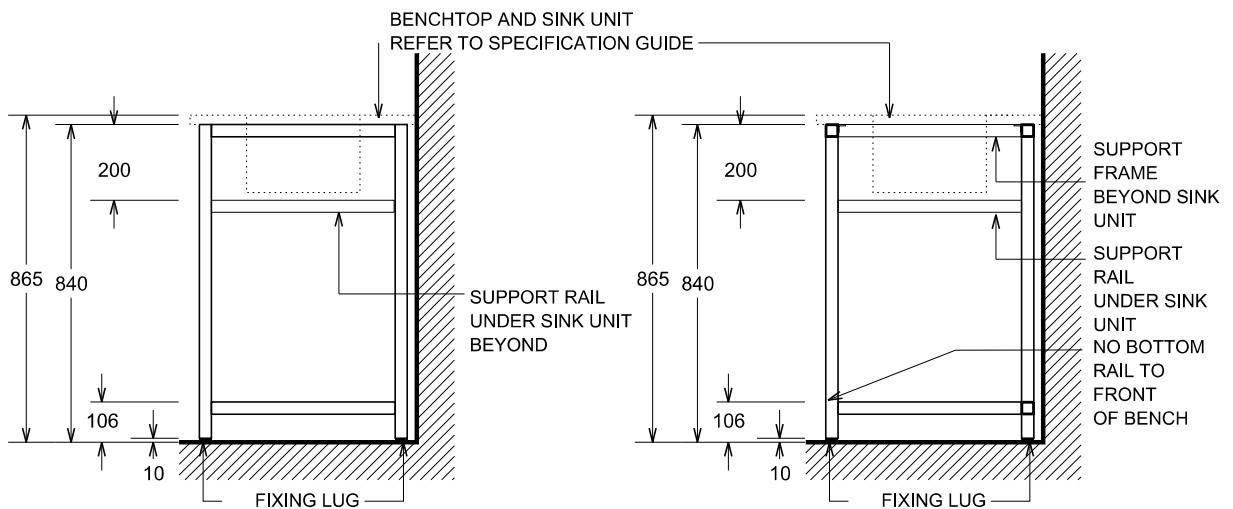
SUPPORT FRAME - END ELEVATION
