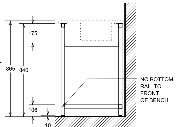
SUPPORT FRAME - SECTION THROUGH TROUGH
