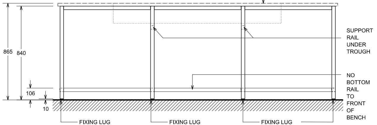
SUPPORT FRAME - FRONT ELEVATION
