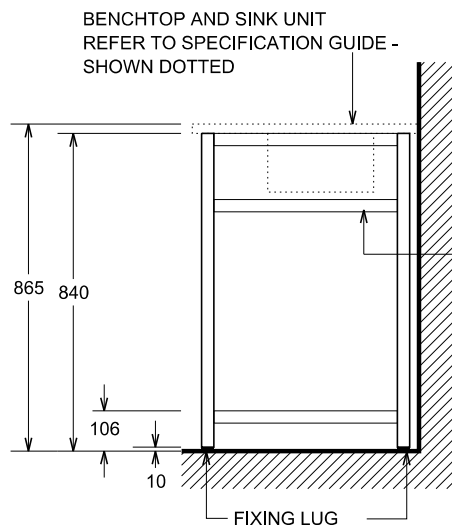
SUPPORT FRAME - END ELEVATION
