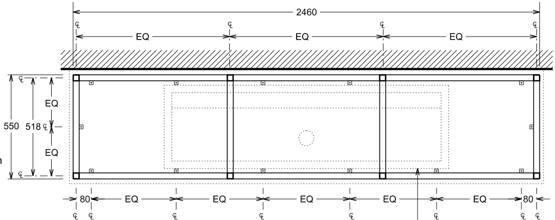
SUPPORT FRAME - PLAN
