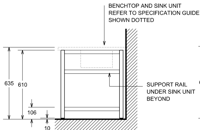
SUPPORT FRAME - END ELEVATION
