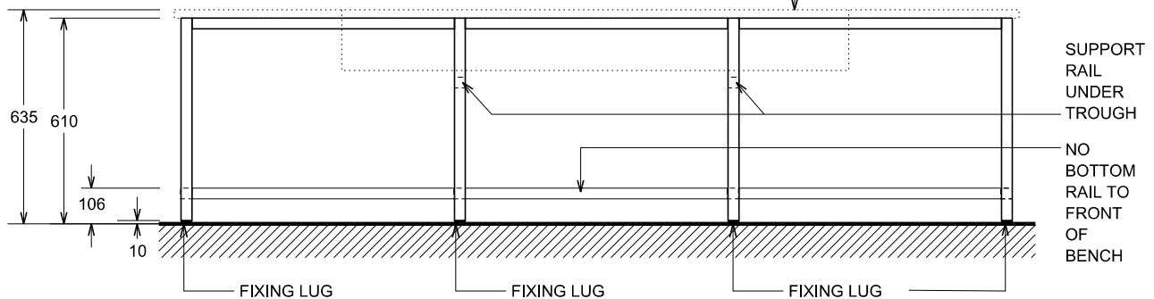
SUPPORT FRAME - FRONT ELEVATION
