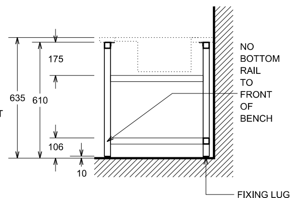
SUPPORT FRAME - SECTION THROUGH TROUGH
