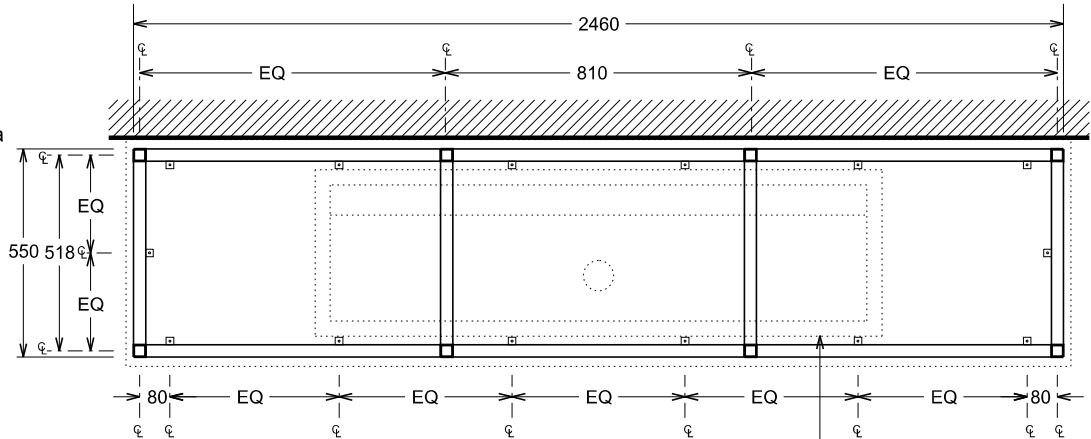
BENCHTOP AND SINK UNIT REFER TO SPECIFICATION GUIDE SHOWN DOTTED
