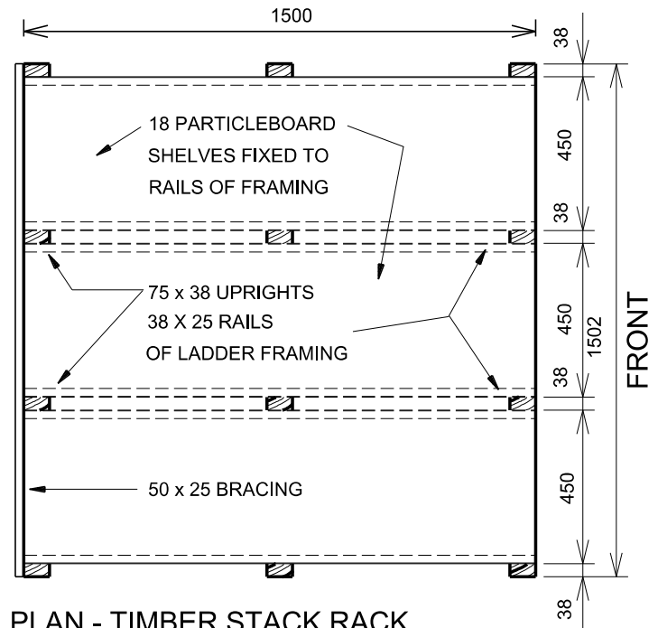
PLAN - TIMBER STACK RACK
