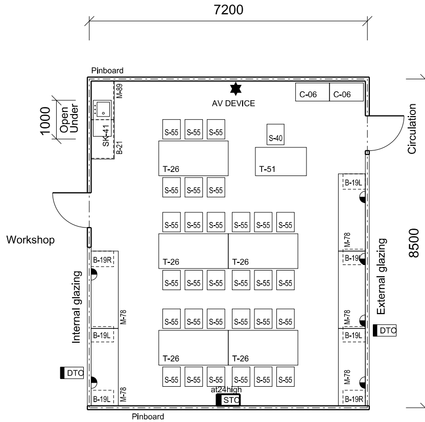
Floor Area shown 59.64 sq.m
