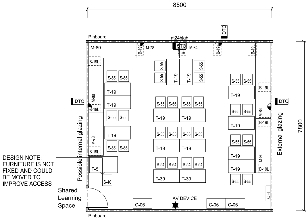
Floor Area shown 64.68 sq.m
